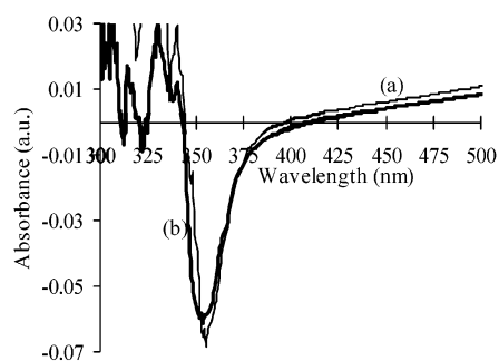
Figure 4. Spectral changes of the (a) bare TiO 2 and (b) SrTiO 3 coated TiO 2 electrodes at applied -0.9 V vs SCE in HClO 4 aqueous solution (pH 1.8). The short wavelength bleach that is related to the electrons accumulation in the TiO 2 is not effected by the coating.
